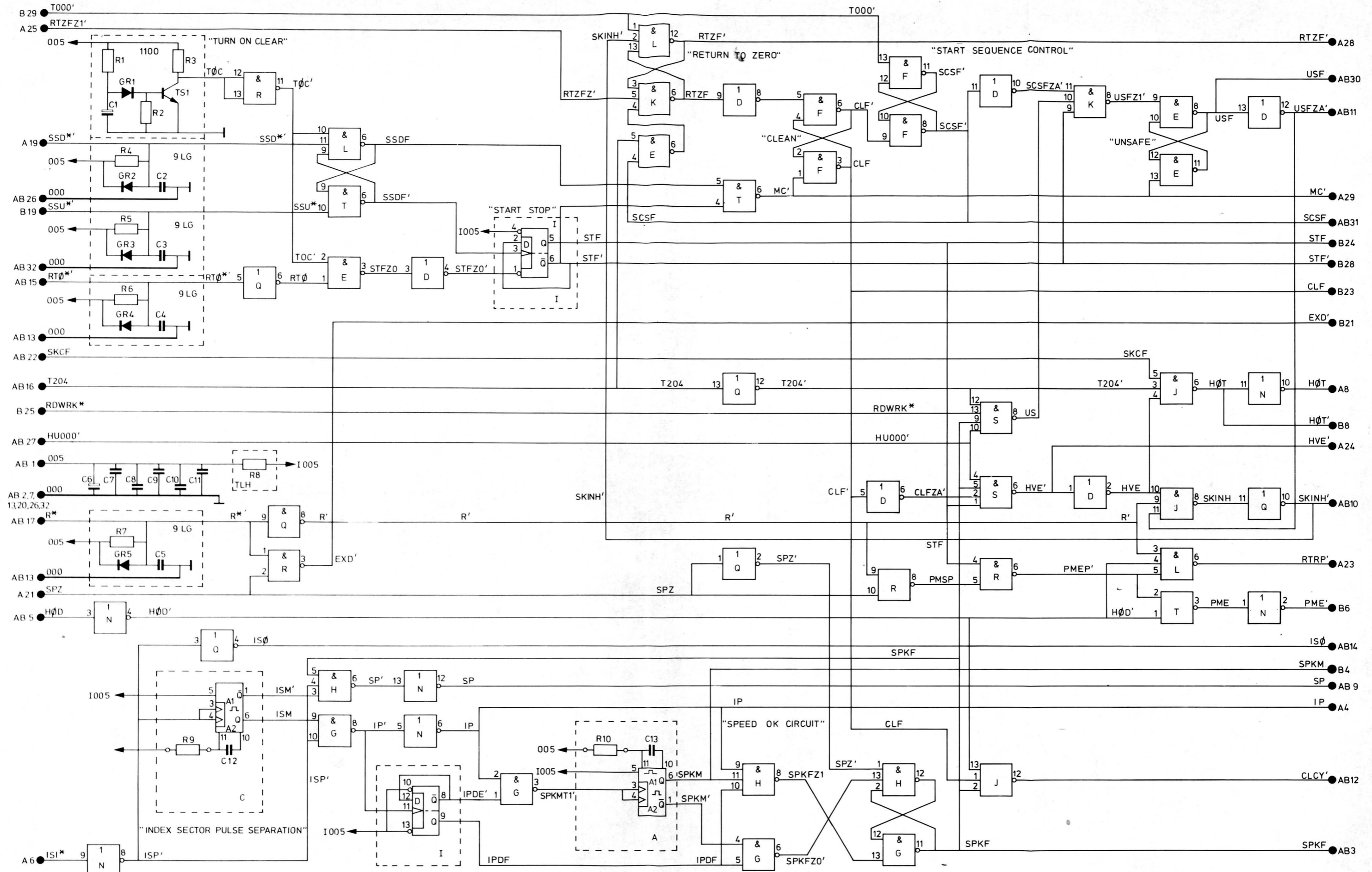
FIG. 3-42 START/STOP/SAFETY CONTROL CARD 9
