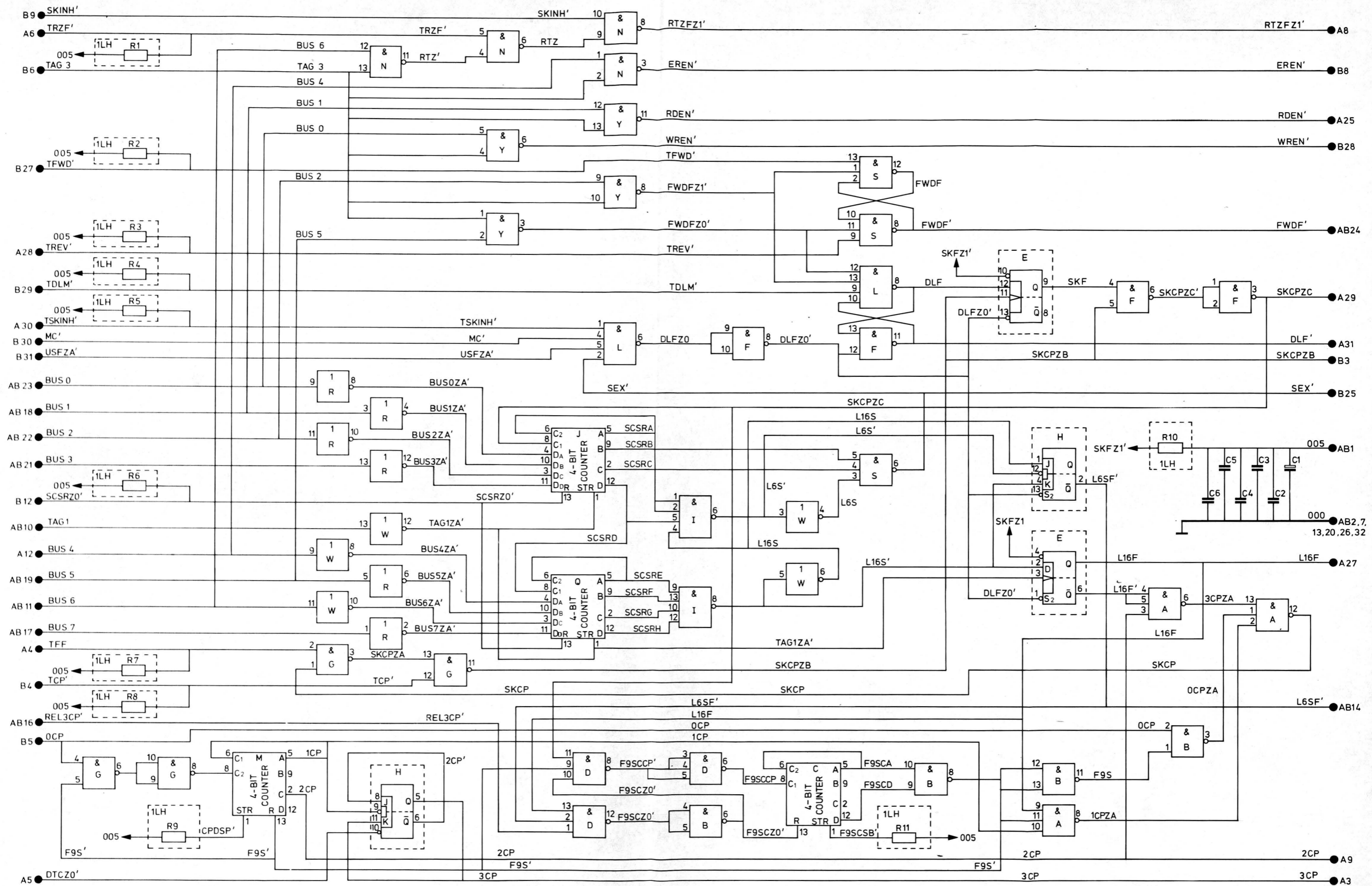
FIG. 3.43 REGISTER VARIABLE SPEED CARD 11
