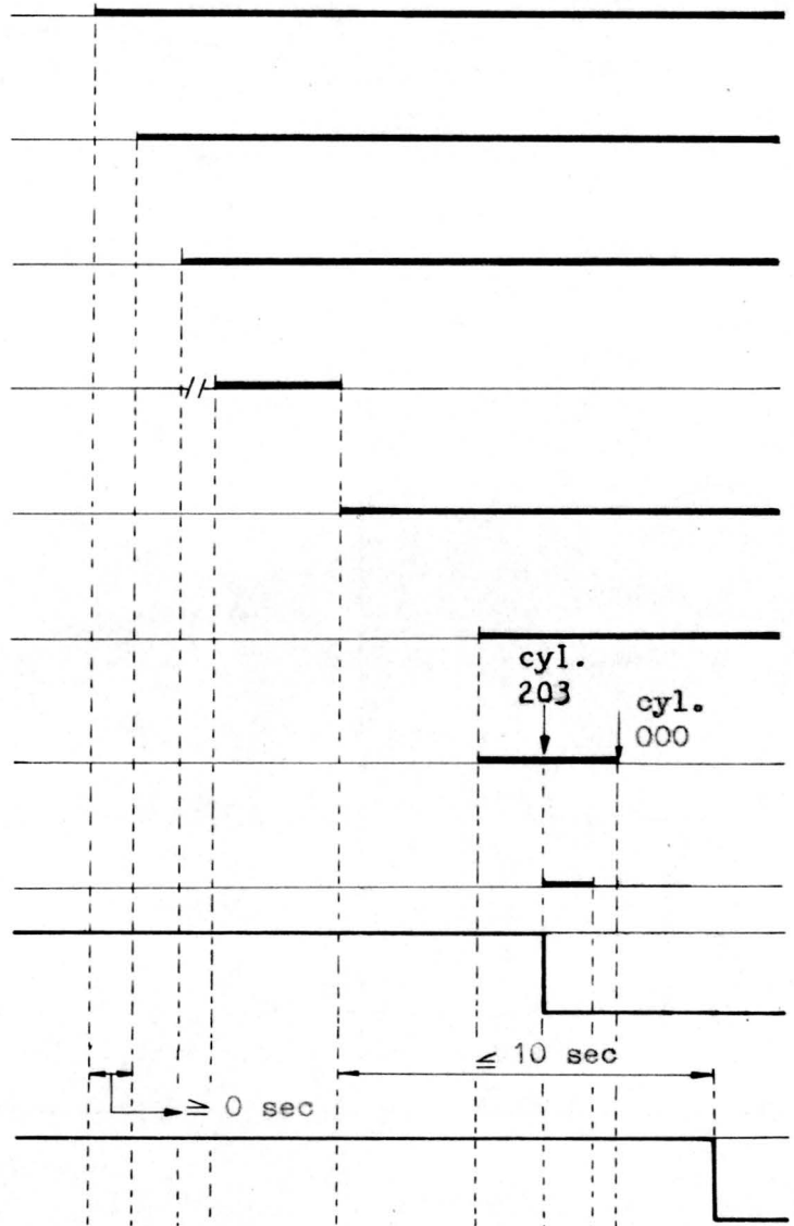
TURN ON TIMING
