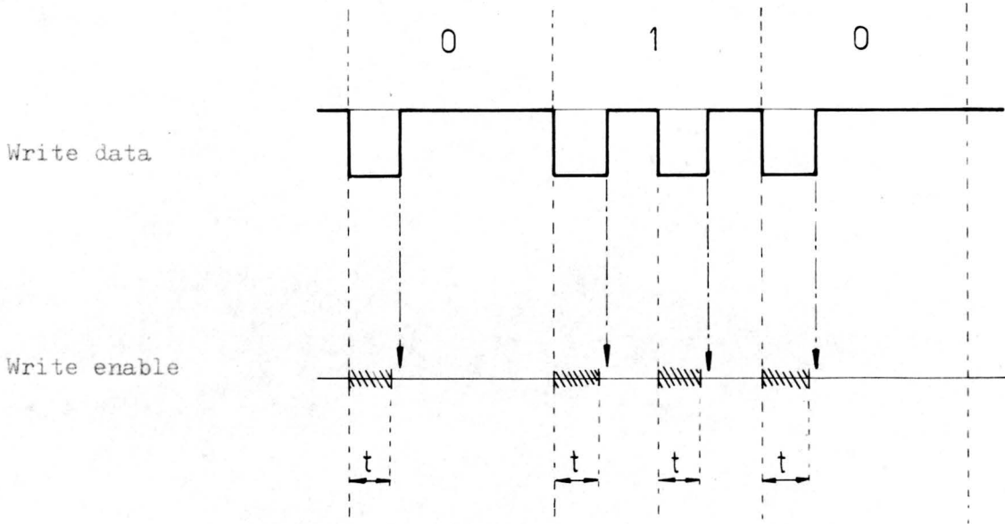
TIMING RELATION WRITE DATA-WRITE ENABLE AT THE END OF A WRITE OPERATION
