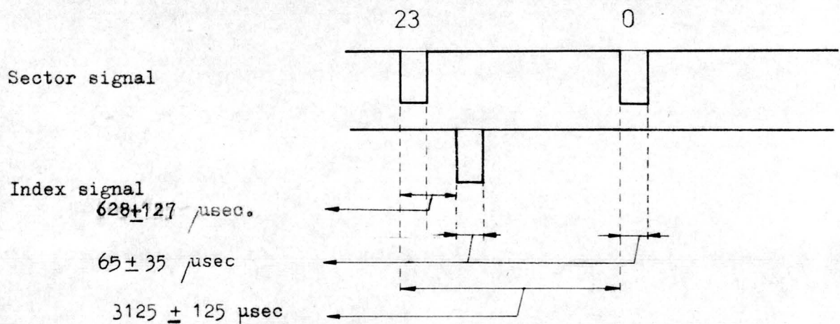
B. timing with 24 sectors
