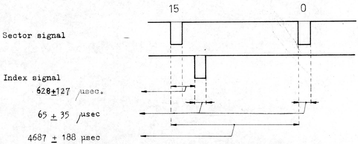
A. timing with 16 sectors
